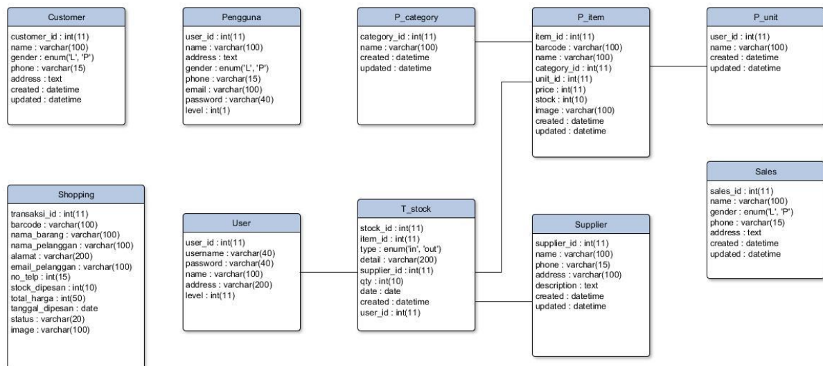
Gambar 6. Class Diagram
