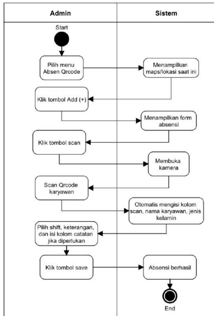
Gambar 3. Activity Diagram Absen
