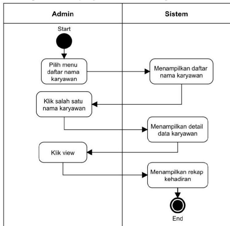
Gambar 6. Activity Diagram Rekap Kehadiran
