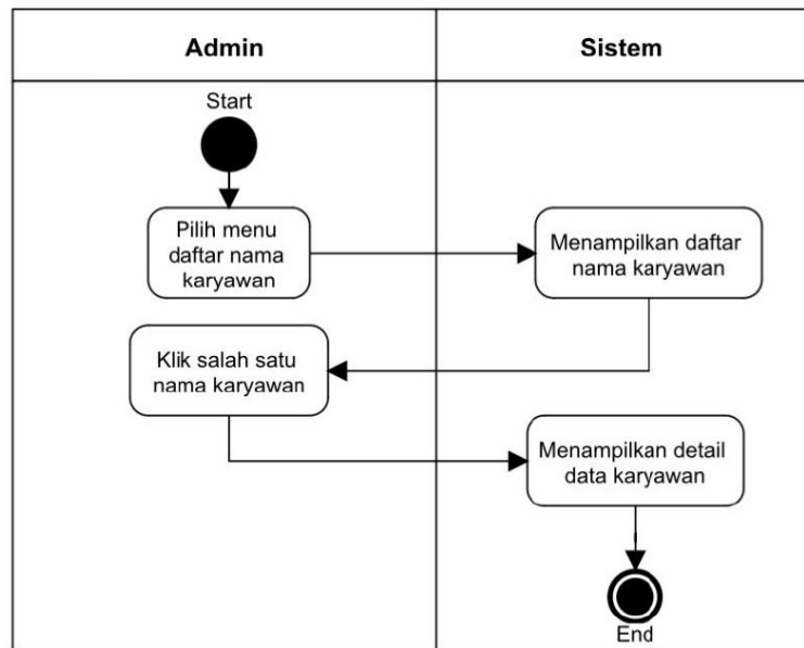
Gambar 5. Activity Diagram Kelola Data Karyawan
