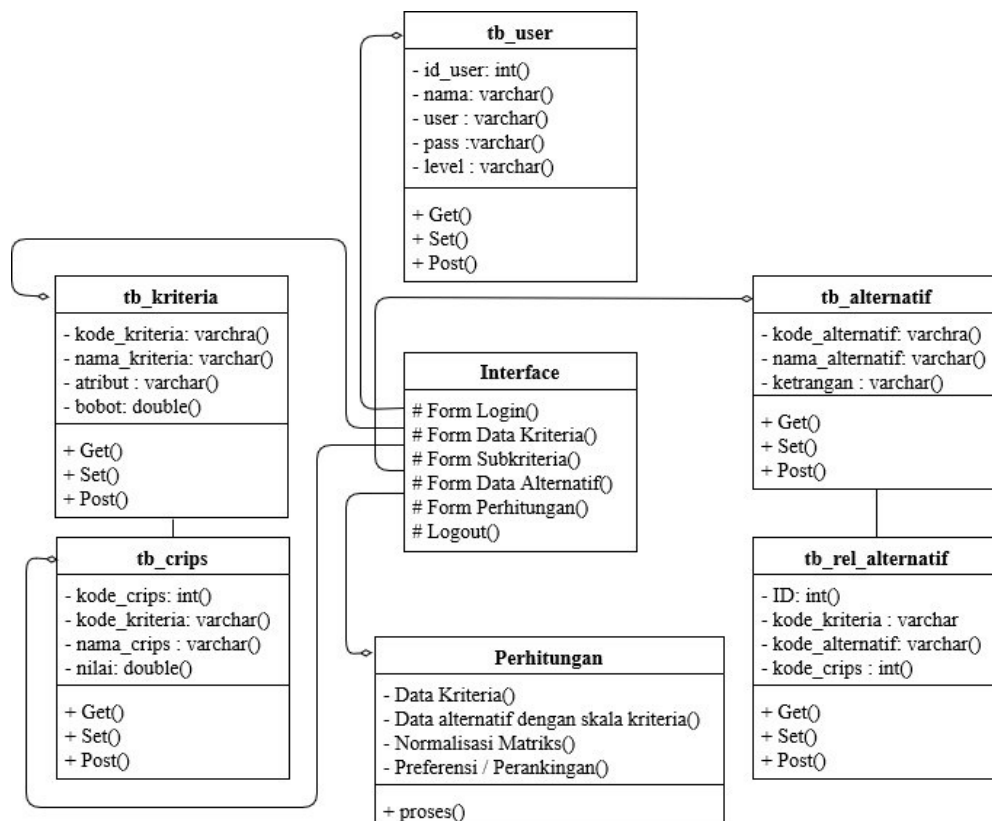
Gambar 5. Class Diagram
